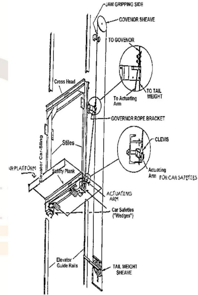
CAR SLING AND PLATFORM OF A TRACTION ELEVATOR DIAGRAM NO. 1
